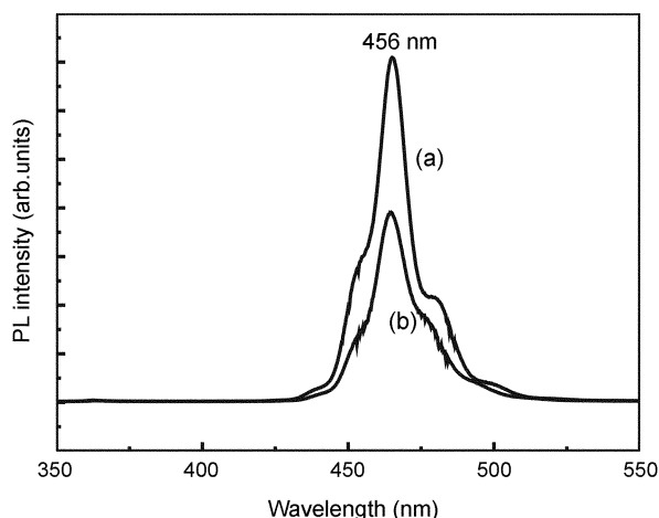
Fig. 3. PL spectra of the InGa x N/GaN triangular MQW structures, measured at room temperature: (a) sample A and (b) sample B.
